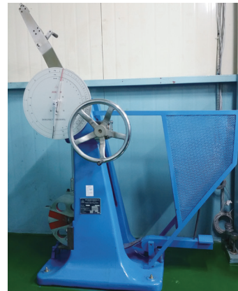
Impact Test Machine
